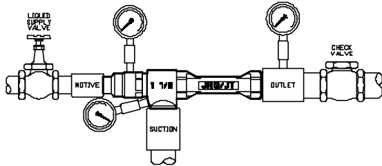
Figure 1: Pumping Liquids
