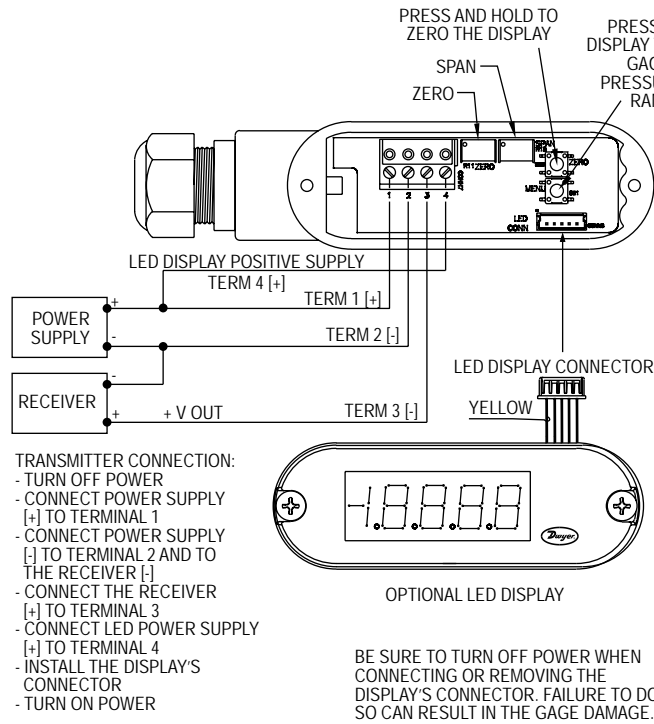
Figure H: Voltage output with optional LED display connection
