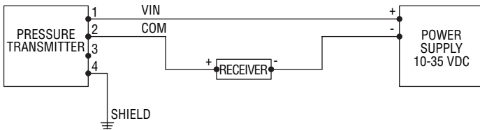
Figure 1: Current Output Connection
