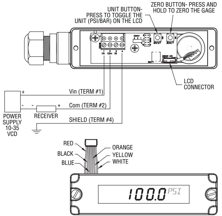
Figure 2: Current Output with Optional LCD
