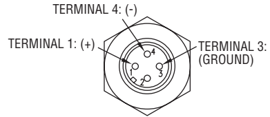
Figure 3: Current Output with Optional M-12 4 Pin Connector
