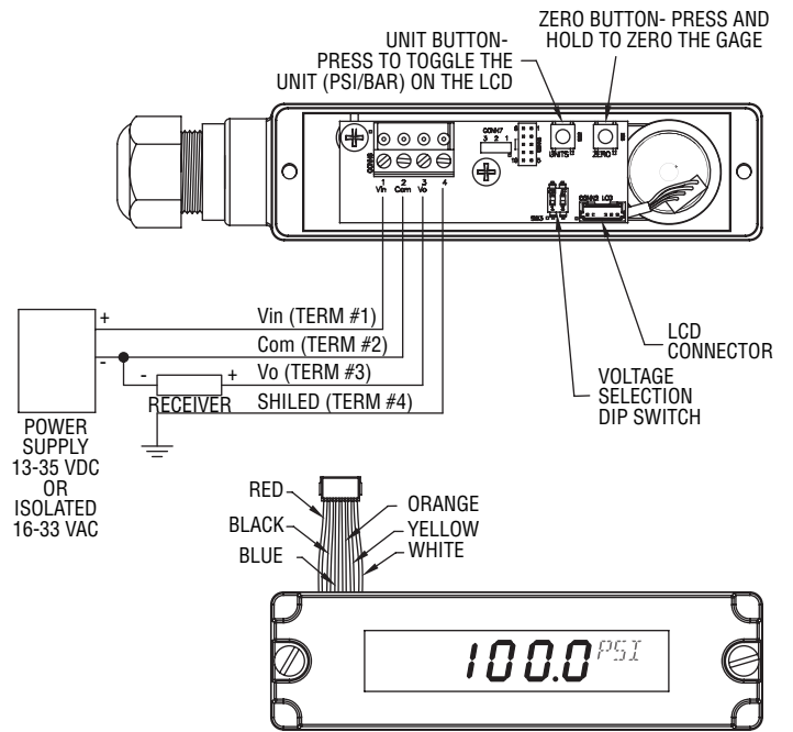
Figure 6: Voltage Output with Optional LCD
