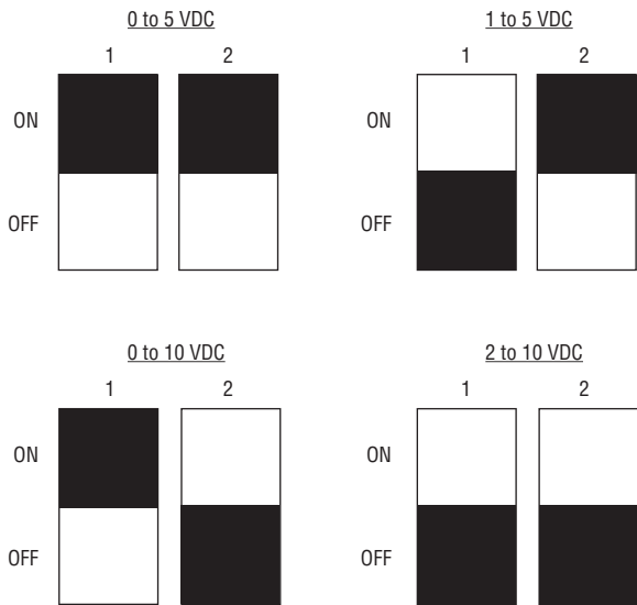
Figure 4: Voltage Output DIP Switch Selection
