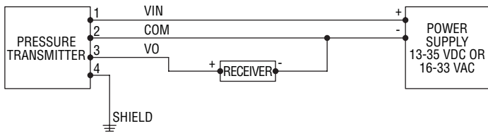
Figure 5: Voltage Output Connection
