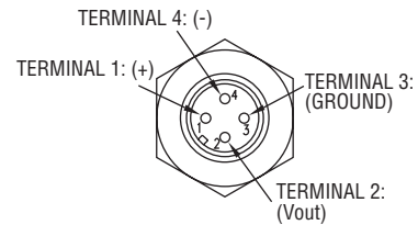
Figure 7: Voltage Output with Optional M-12 4 Pin Connector
