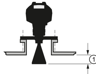
Hygienic encapsulated antenna (HEA)
