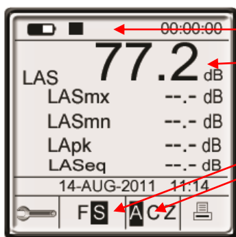
Figure 2-2: Measurement screen displaying multiple measurements
