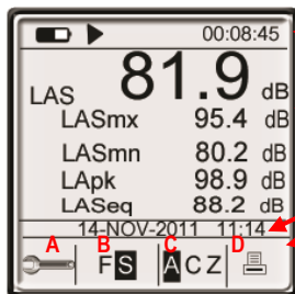
Figure 1-1: SE-400 Series Screen
