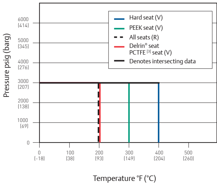
Pressure vs. Temperature - Brass valves
