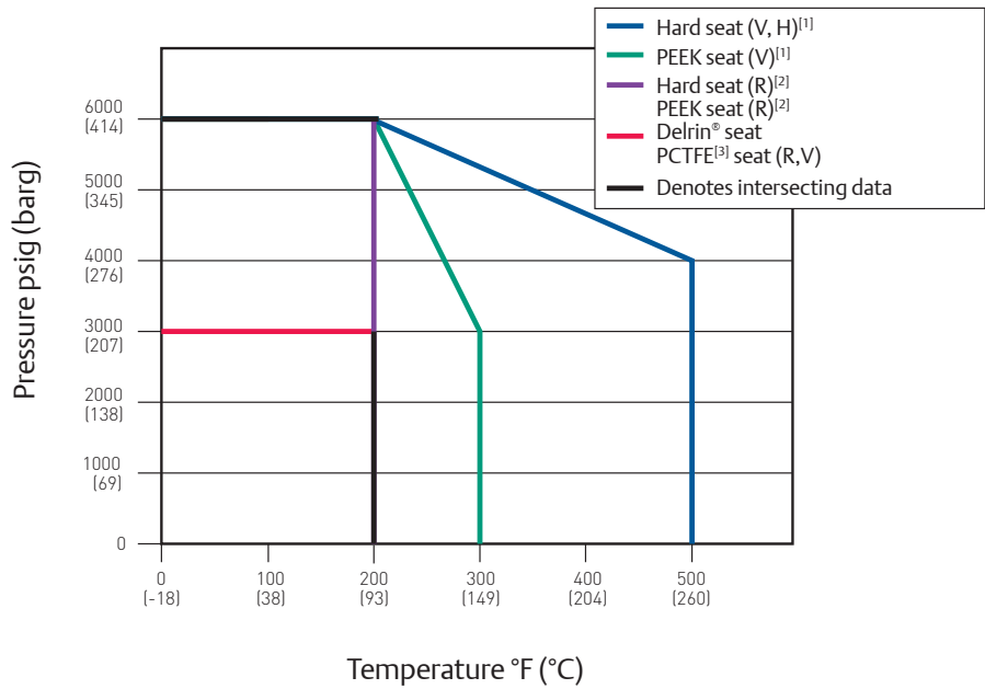
Pressure vs. Temperature - CS and 316 SS valves
