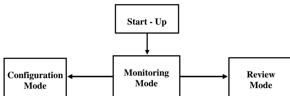
Diagram 12: Mode Structure
