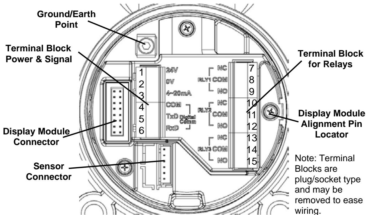
Diagram 7: Terminal module
