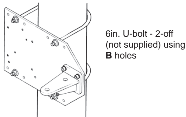
Mounting Plate Fixed to Single Pipe/Pole
