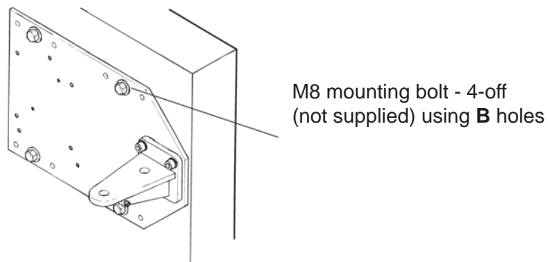
Mounting Plate Fixed to Flat Surface
