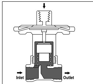
Figure 11A: Normally Open, Operator Exhausted
