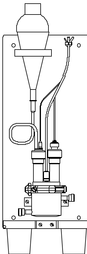
High Purity Electrode Mounting Assembly (Panel Mounted Option)
