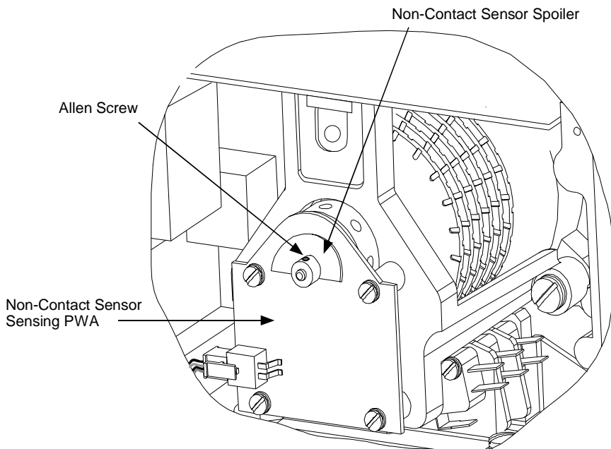
Figure 3 Non-Contact Sensor Assembly
