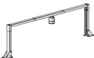
FMS-350 Bridge Channel Bracket, Floor Mount
